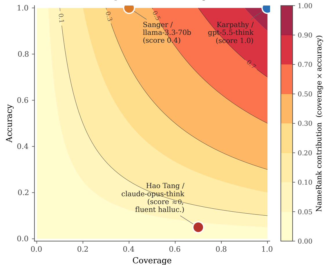
(a) Contribution = cov \times acc: fluent hallucinations collapse on the bottom edge.
