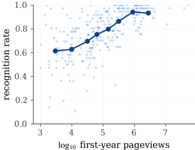
(a) Dose-response ( R^2=0.39 )
