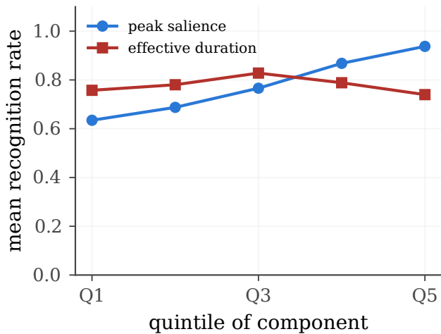
(b) How loud, not how long
