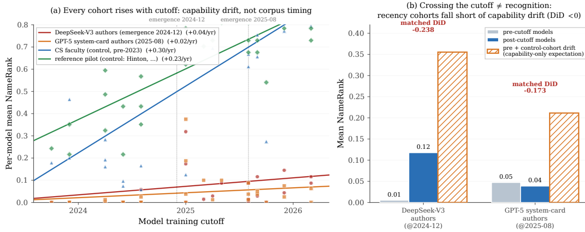
Figure 13. Training-cutoff gradient. (a) Per-model mean NameRank vs. training cutoff for two first-appearance “recency” cohorts (DeepSeek-V3 authors, emergence 2024-12; GPT-5 system-card authors, 2025-08) and two stable controls nameable since well before any cutoff. Every cohort rises with cutoff at \sim 0.1\text{--}0.3/\text{yr} —a model-capability confound, not corpus timing (one control cohort contains Geoffrey Hinton). (b) Natural experiment: the recency cohorts’ pre/post-emergence jump is smaller than the same-split jump on the stable controls (hatched “capability-only expectation” bar), so the matched difference-in-differences is negative ( -0.24 , -0.17 ). Crossing a model’s training cutoff is necessary but far from sufficient for recognition.
