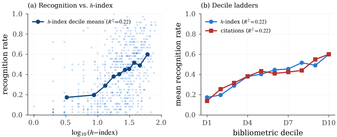
Figure 7. Bibliometric predictors. (a) Recognition vs. \log_{10}(h\text{-index}) for OpenAlex researchers, with decile means. (b) Decile ladders for h\text{-index} and raw citations: both rise with productivity, neither dominates, and both leave most variance unexplained.
