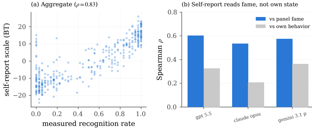
Figure 11. Introspection reads the corpus prior. (a) Bradley–Terry self-report scale vs. measured panel recognition: the ordering is recovered fairly well in aggregate. (b) But per model, self-report tracks cross-panel fame far better than the model’s own behavioral record—it reads what everyone knows, not its own weights.
