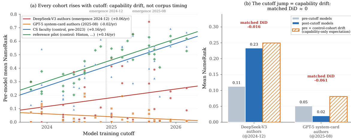
Figure 8. Training-cutoff gradient. (a) Per-model mean NameRank vs. training cutoff for two first-appearance “recency” cohorts (DeepSeek-V3 authors, emergence 2024-12; GPT-5 system-card authors, 2025-08) and two stable controls nameable since well before any cutoff. Every cohort rises with cutoff at \sim 0.10 – 0.20/\text{yr} —a model-capability confound, not corpus timing (one control cohort contains Geoffrey Hinton). (b) Natural experiment: the recency cohorts’ pre/post-emergence jump matches the same-split jump on the stable controls (hatched “capability-only expectation” bar), so the matched difference-in-differences is \approx 0 . Crossing a model’s training cutoff is necessary but not sufficient for recognition.
