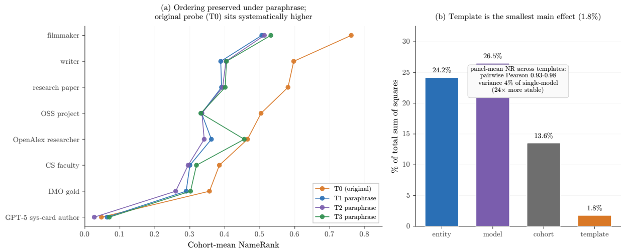
Figure 14: Prompt-paraphrase sensitivity (cohort-stratified 200-entity subset, 37-model panel, 4 templates, 29,600 records). (a) Cohort-mean NameRank under the original probe (T0) and three paraphrases (T1–T3). The cohort ordering is preserved (pairwise Pearson 0.93–0.98), but T0 sits systematically higher—the absolute level is wording-specific. (b) Additive variance decomposition: template is the smallest main effect (1.78% of total SS), and the panel-mean NameRank across templates is 24\times more stable than a single model at a single template.
