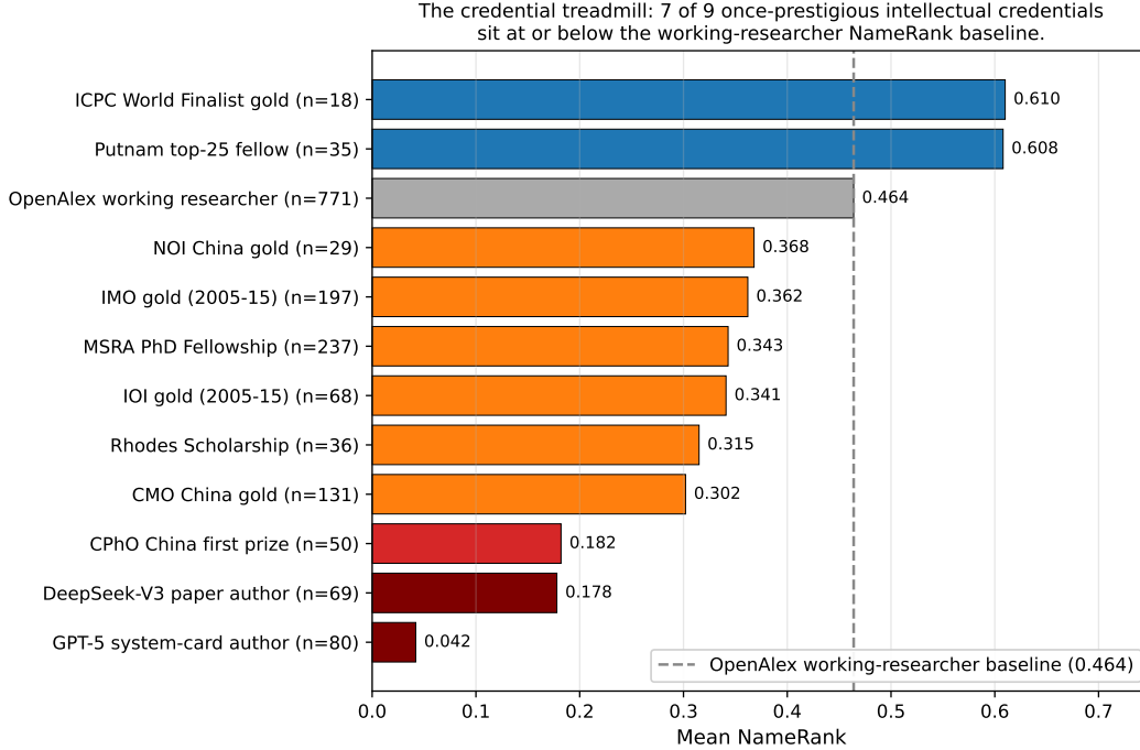
Figure 2: The credential treadmill (graphical form of Table 3). Bars are cohort mean NameRank; the dashed grey line is the long-tail-OpenAlex working-researcher baseline (0.464). Red bars: silent or near-silent cohorts. Orange: at or just below the baseline. Blue: above the baseline. Of nine prestigious-credential cohorts, only two (ICPC, Putnam) clear the working-researcher baseline.
