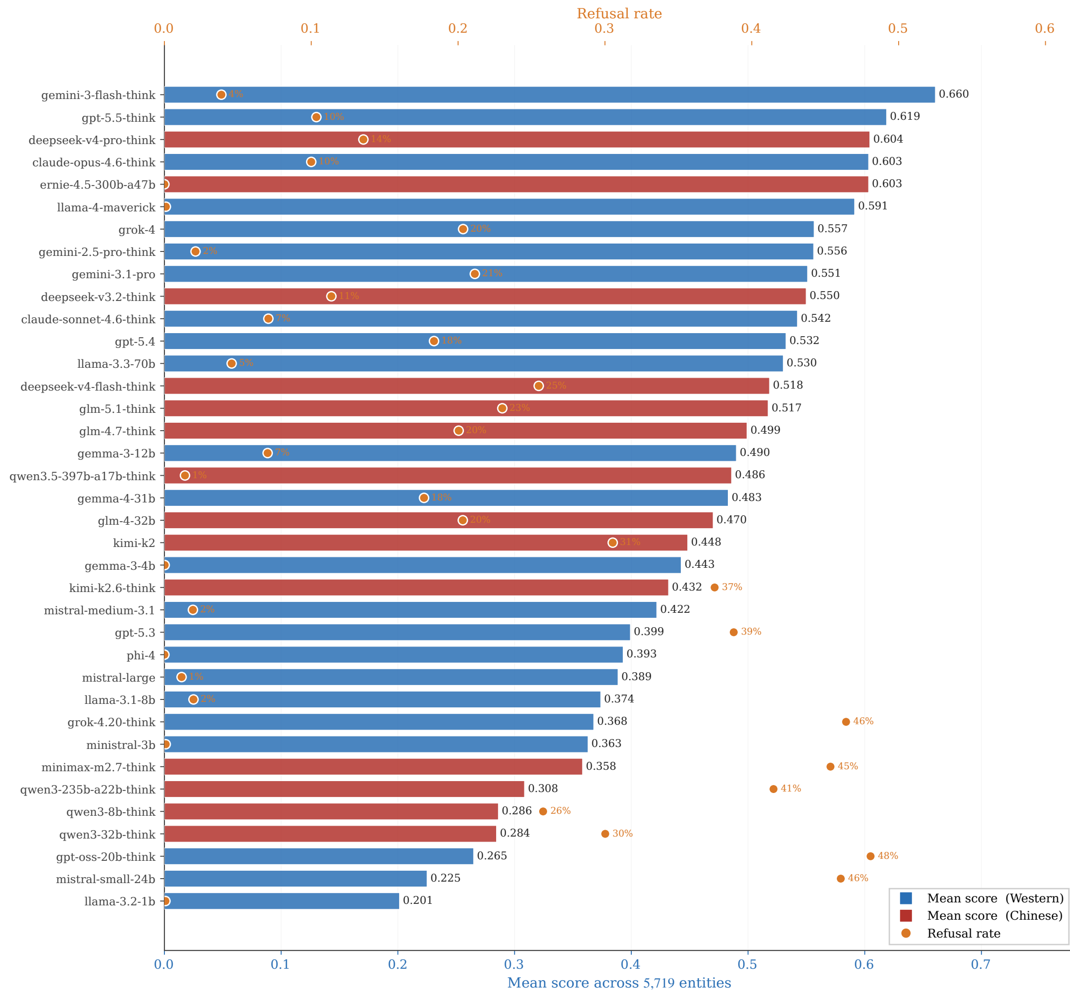
Per-model generosity and refusal across the 37-model panel (graphical form of Table~3, Appendix~C). Sorted by mean score.
