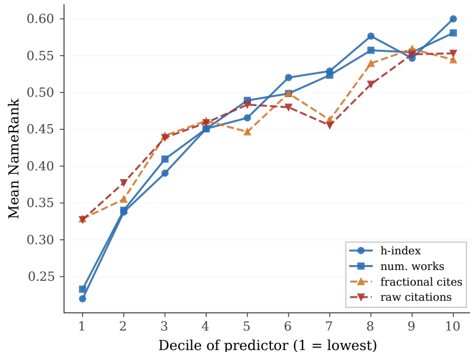
(b) h -index and works-count rise steeply; fractional cites track raw cites
