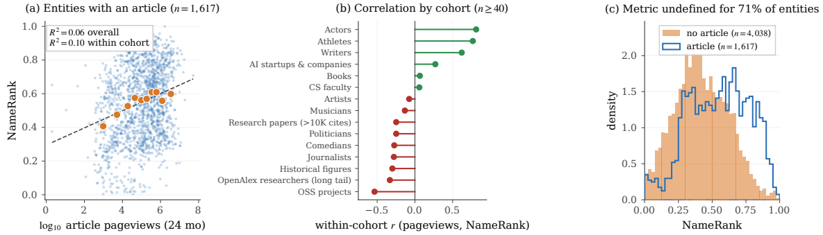
Figure 11. NameRank is not Wikipedia-pageview rank. (a) NameRank against \log_{10} 24-month article pageviews for the 1,617 entities with a resolvable article (small dots: entities; large markers: decile means): R^2 = 0.06 overall, 0.10 within cohort. (b) Within-cohort correlation for cohorts with n \geq 40 matched entities: positive only for celebrity cohorts, negative for technical and production cohorts—current attention flow vs. accumulated corpus stock. (c) NameRank distribution for entities with and without an article: the attention metric is undefined for the 71% without one, whose scores span the discriminative zone.
