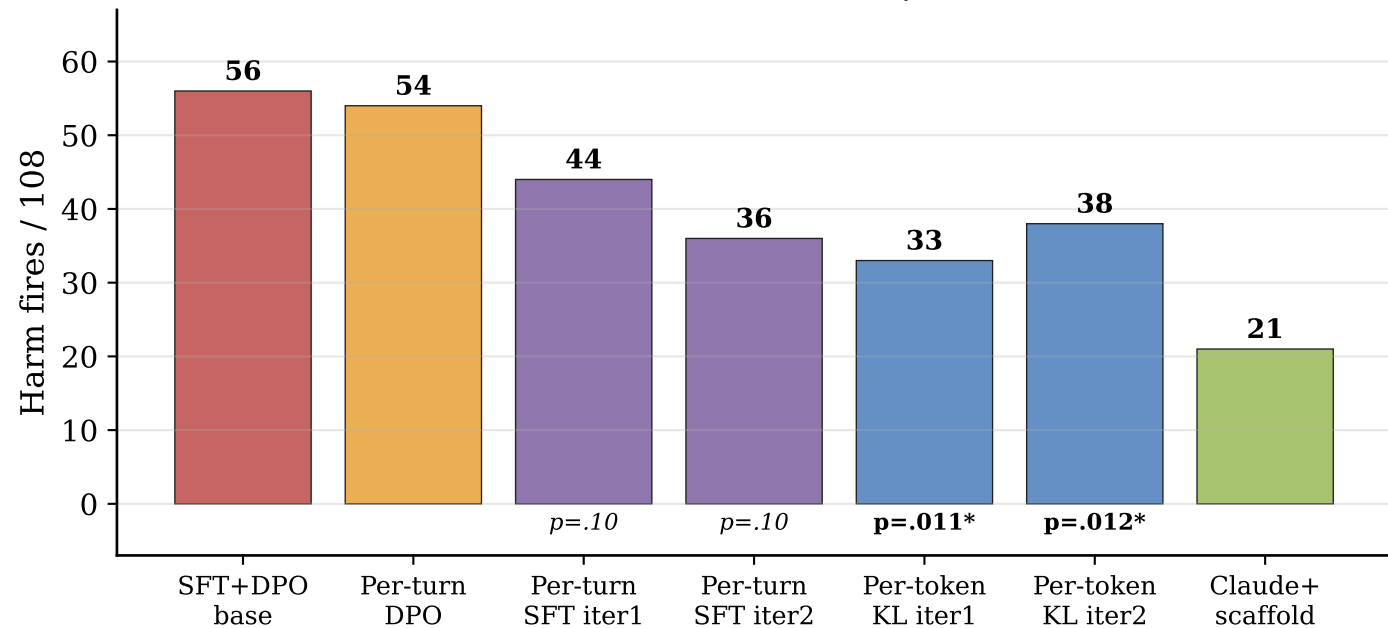
Distillation variant ladder on Qwen3-8B (*: p < 0.05 vs SFT+DPO base)
