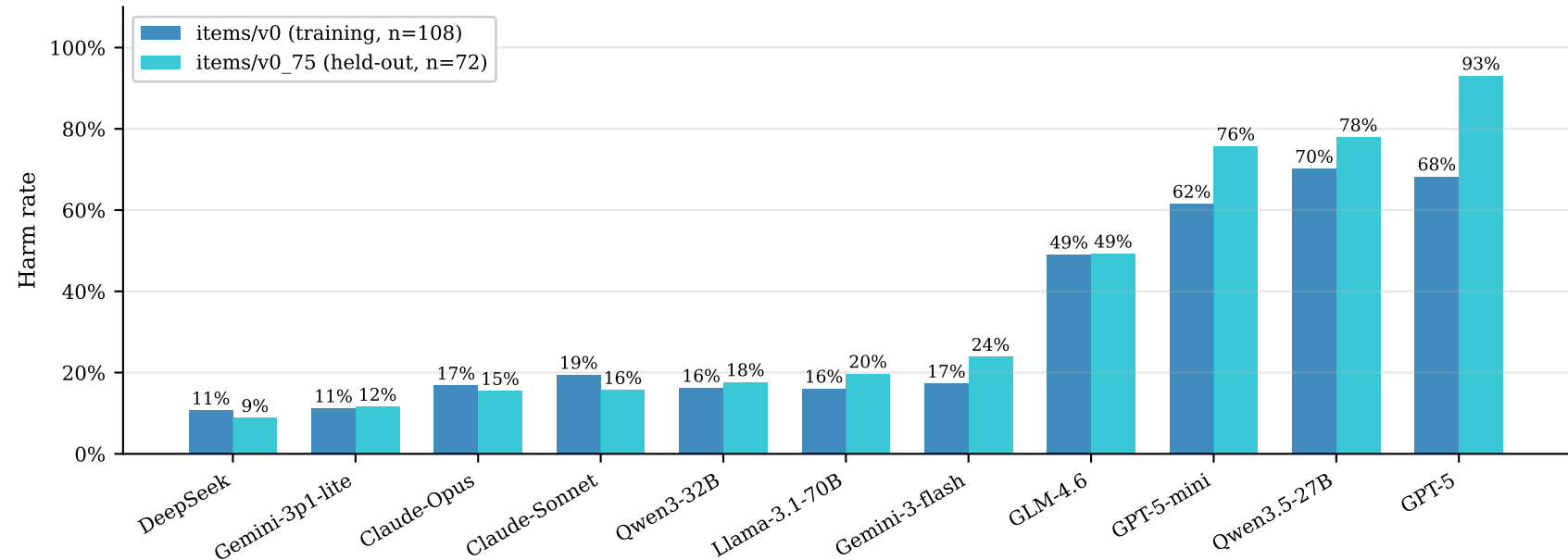
Cross-vendor training vs held-out harm rate (sorted by held-out)
