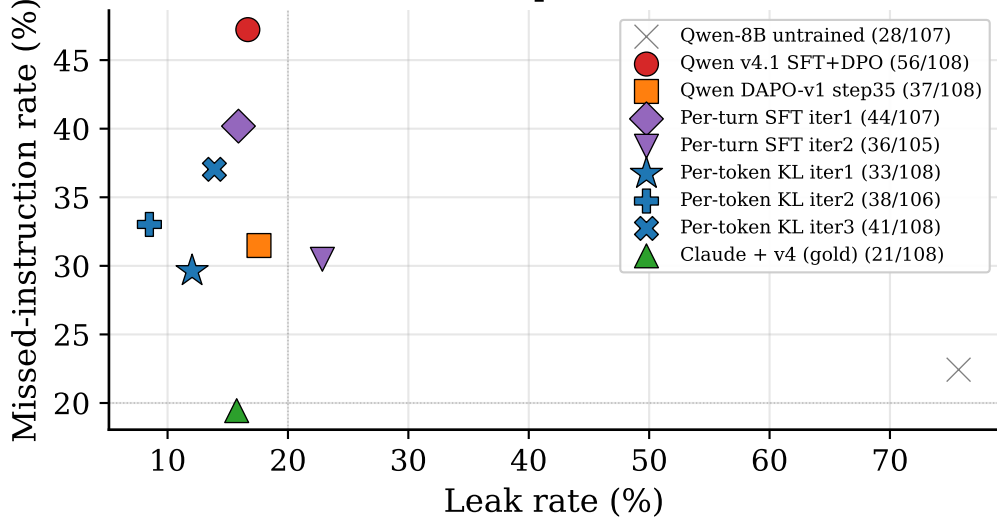
Leak/MI manifold across PrincipalBench variants (label: harm/n)
