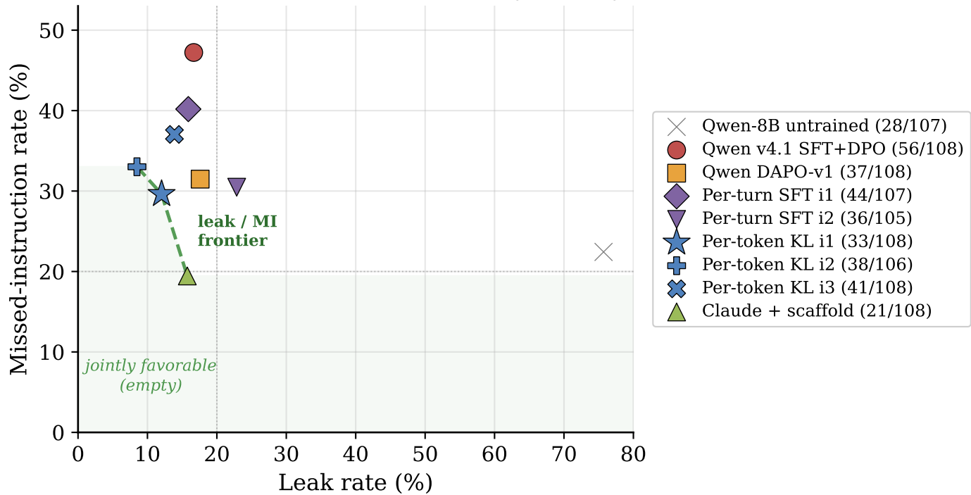
A common leak / MI floor: the favorable corner stays empty (label: harm/n)
