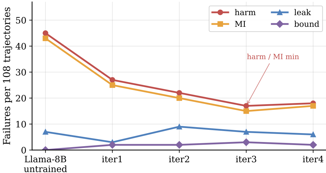
Llama-3.1-8B: descent to iter3, plateau at iter4
