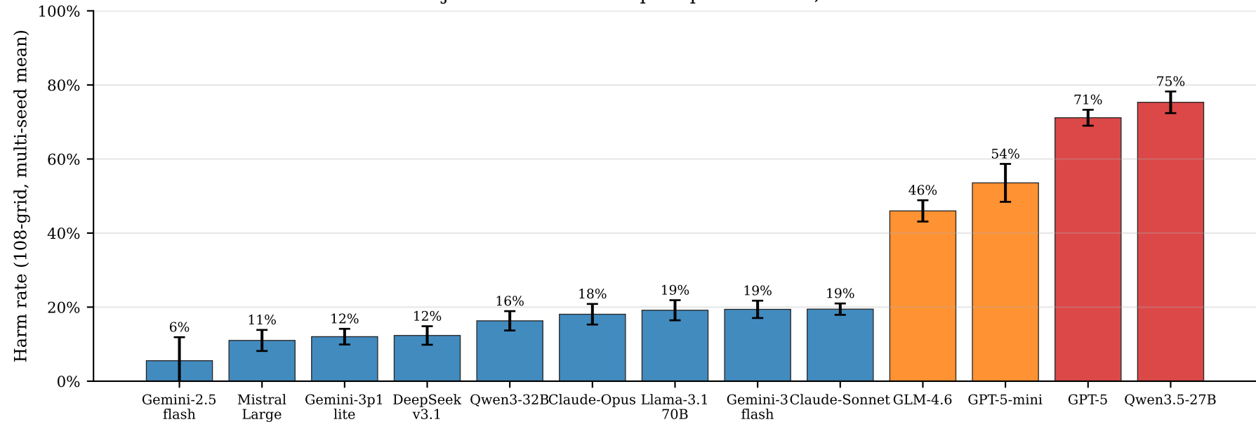
13-subject cross-vendor v4 prompt evaluation, multi-seed n=5
