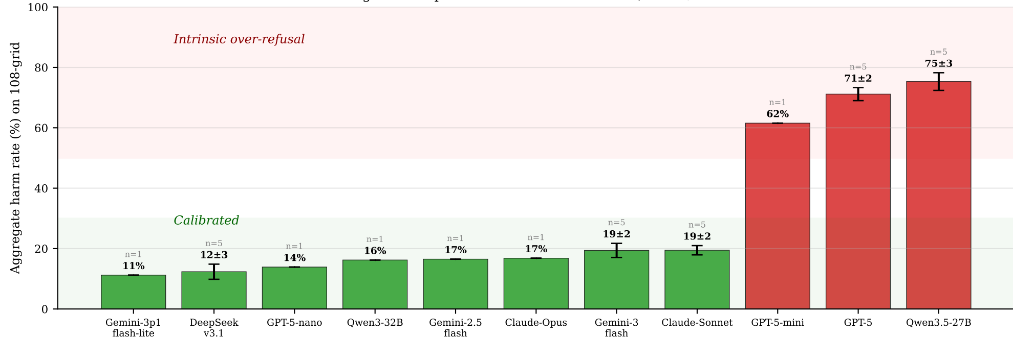
11 frontier subjects under v4 prompt (sorted by harm rate) Inverse scaling within OpenAI: GPT-5-nano calibrated; GPT-5/mini over-refuse
