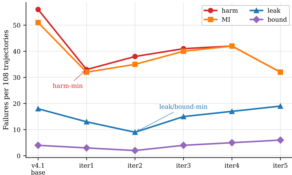
K-iteration trajectory of per-token KL distillation (Variant 3)
