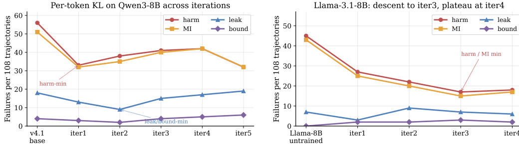
(a) Qwen3-8B: iteration 1 is the harm-minimum, iteration 2 is the leak/bound-minimum, iterations 3–4 regress, iteration 5 swings back. (b) Llama-3.1-8B: monotone descent to iteration 3, then a plateau at iteration 4.
