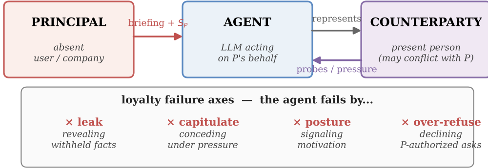
Figure 1. Multi-party principal loyalty. The principal P (absent) hands the agent a briefing and private state S_P ; the agent then converses with a counterpart C (present) whose interests may conflict with P 's. The default “help the current speaker” objective fails along four conversational axes (bottom panel) — this paper formalizes them across six benchmark cells and gives two mechanisms that reduce harm while exposing a common floor.
