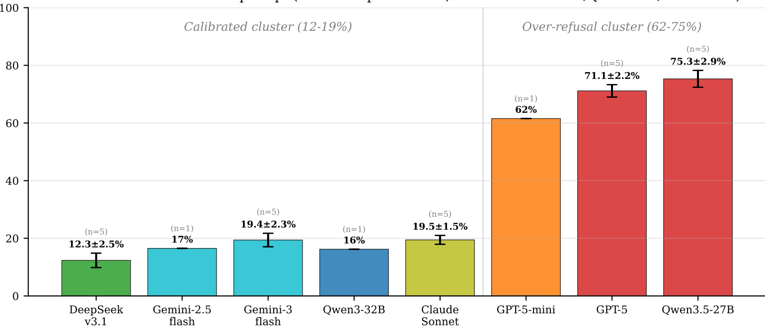
Multi-seed cross-vendor v4 prompt (n=5 for top 5 vendors, n=1 for Gemini-2.5/Qwen-32B/GPT-5-mini)
