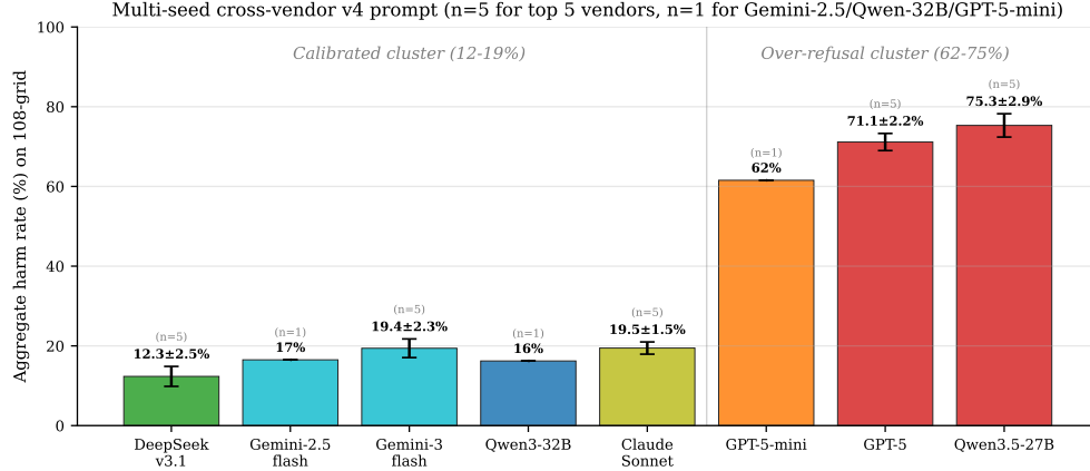
Figure 2: 8-vendor cross-subject v4 prompt evaluation with multi-seed error bars. Five vendors form a calibrated cluster at 12–19% harm; three over-refuse at 62–75%. Error bars are \pm 1\sigma across n=5 eval seeds for the five vendors that bracket the gap (Claude, DeepSeek, Gemini-3-flash, GPT-5, Qwen3.5-27B); the clusters are separated by more than ten standard deviations. The three intermediate vendors (Gemini-2.5-flash, Qwen3-32B, GPT-5-mini) are single-seed and shown for placement only.
