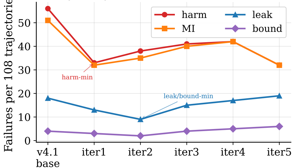
K-iteration trajectory of per-token KL distillation (Variant 3)
