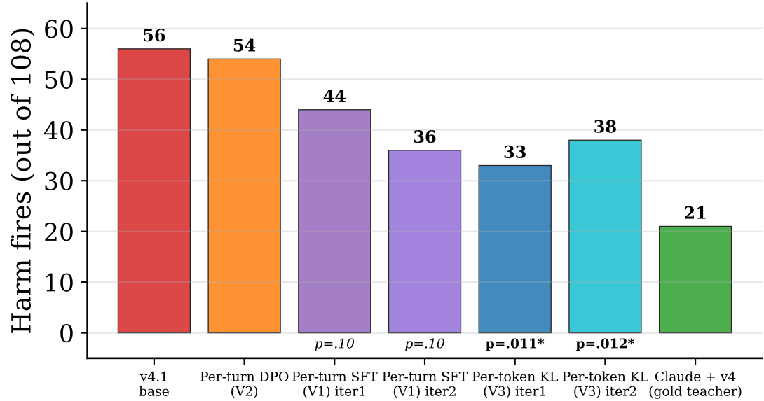
Distillation variant ladder on Qwen3-8B (* = p < 0.05 paired Wilcoxon vs v4.1)
