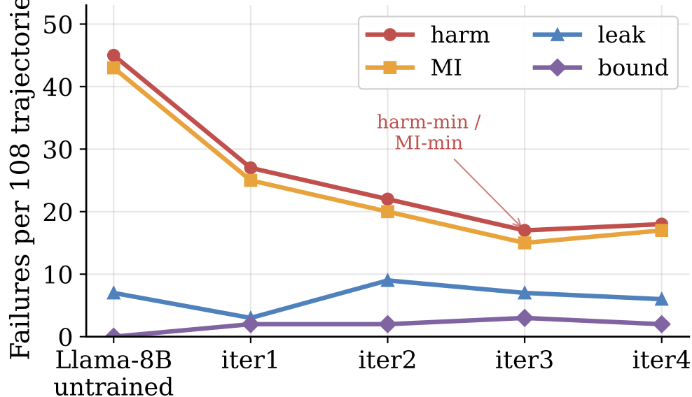
Llama-3.1-8B: monotone descent to iter3, then plateau
