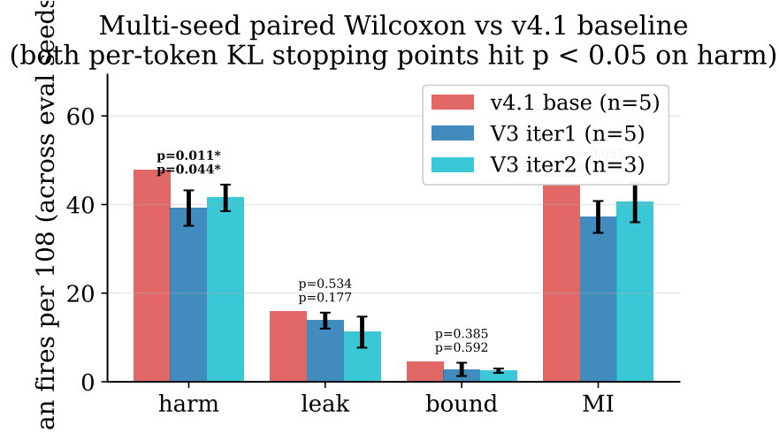
Figure 7. Multi-seed paired Wilcoxon vs. the SFT+DPO base. Both per-token-KL stopping points (iteration 1, the harm-minimum; iteration 2, the leak/bound-minimum) reach p < 0.05 on harm. Error bars are \pm 1\sigma across seeds.
