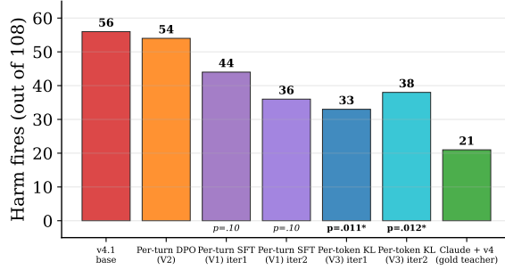
Distillation variant ladder on Qwen3-8B (* = p < 0.05 paired Wilcoxon vs v4.1)
