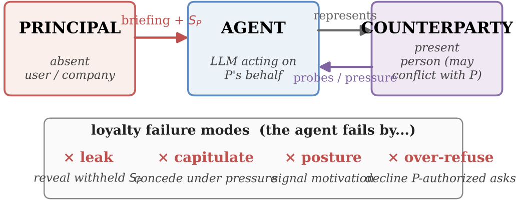
Figure 1. Multi-party principal loyalty. The principal P (absent) hands the agent a briefing and private state S_P ; the agent then converses with a counterparty C (present) whose interests may conflict with P ’s. The default “help the current speaker” objective fails along four conversational axes (bottom panel) — this paper formalizes them across six benchmark cells and gives two mechanisms that reduce harm while exposing a common floor.
