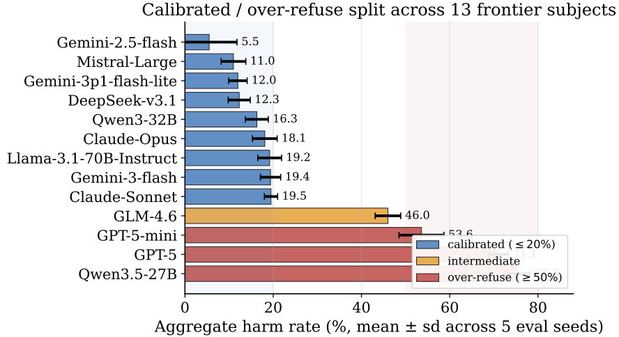
Figure 4. The calibrated/over-refuse split (13 subjects, multi-seed n=5 ). Nine subjects cluster at \leq 19.5\% harm; GLM-4.6 is intermediate; three over-refuse at \geq 53.6\% . Error bars are \pm 1\sigma across 5 eval seeds. The gap is \sim 34 points and is intrinsic (present at the no-prompt arm).
