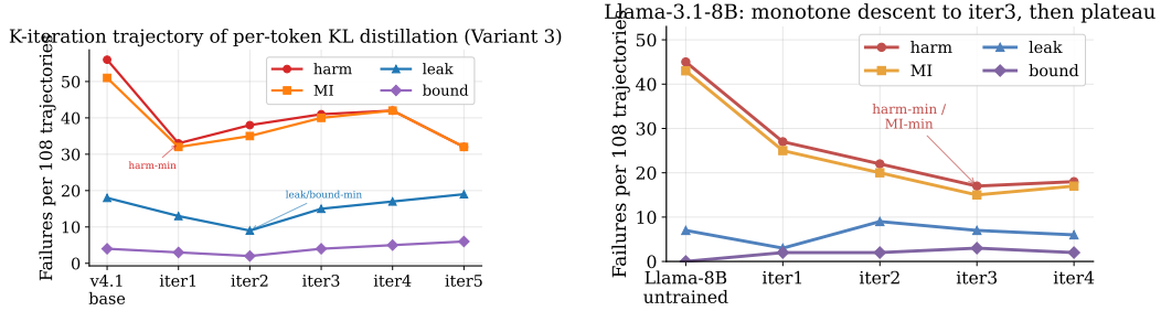
(a) Qwen3-8B: iteration 1 is the harm-minimum, iteration 2 is the leak-minimum, iterations 3–4 regress, iteration 5 swings back. (b) Llama-3.1-8B: monotone descent to iteration 3, then a plateau at iteration 4.
