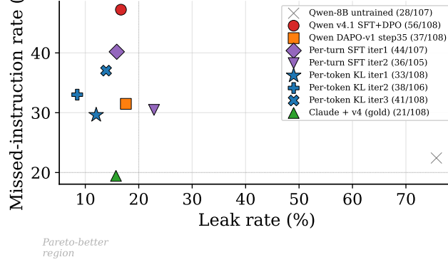
Leak/MI manifold across PrincipalBench variants (label: harm/n)
