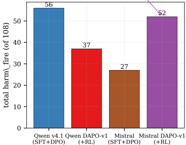
DAPO regresses on Mistral (a) Total harm by base \times stage
