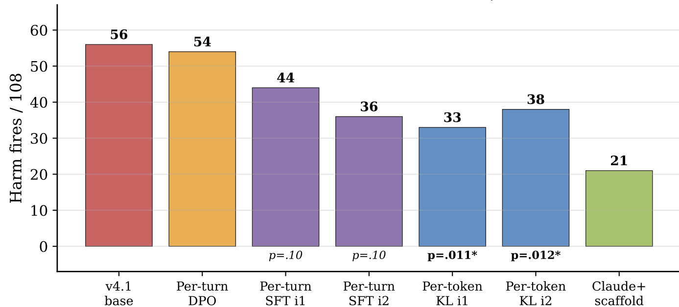
Distillation variant ladder on Qwen3-8B (*: p < 0.05 vs v4.1)
