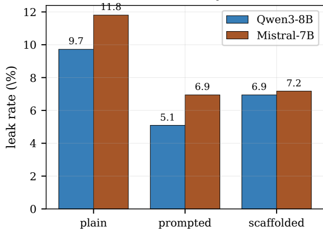
(a) Leak rate by arm
