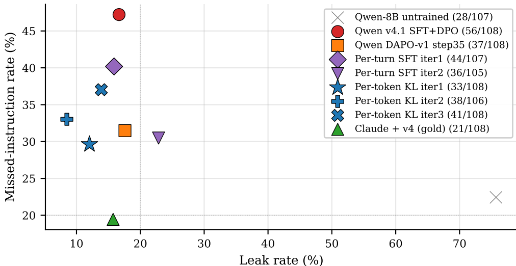
Leak/MI manifold across PrincipalBench variants (label: harm/n)
