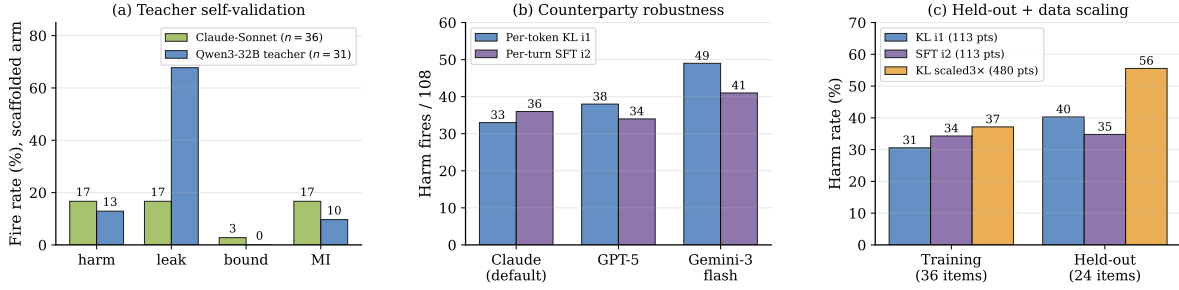
Figure 9. Teacher validation and student robustness (per-token-KL iteration 1 unless noted). (a) The open Qwen3-32B teacher matches Claude-Sonnet on harm and missed-instruction but leaks much more. (b) Swapping the counterparty model raises harm for both variants; per-token KL is somewhat more counterparty-sensitive than per-turn SFT. (c) Per-token KL has the lowest training harm but the largest train-to-held-out gap, and naive 3\times data scaling regresses on held-out.
