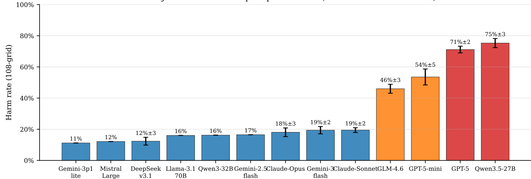
13-subject cross-vendor v4 prompt evaluation (multi-seed where available)
