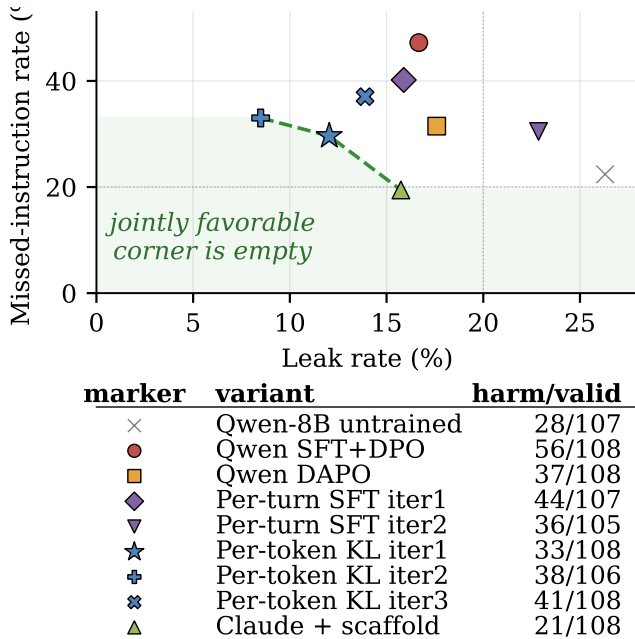
Figure 1: Shared leakage/over-refusal frontier. Inference-time scaffolding and model post-training produce different operating points, but no tested variant reaches the shaded low-leak, low-refusal corner. In the labels, iter1 , iter2 , and iter3 denote successive post-training iterations; the key reports harm/valid cells.
