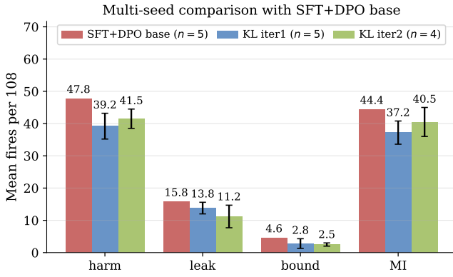
Figure 5: Multi-seed model post-training improvement. Against the SFT+DPO base, per-token-KL iteration 1 has the lowest mean harm (47.8 \rightarrow 39.2) and missed-instruction count (44.4 \rightarrow 37.2), whereas iteration 2 has the lowest mean leak (15.8 \rightarrow 11.2) and private-bound count (4.6 \rightarrow 2.5). Bars show mean failures per 108 cells; error bars show \pm 1\sigma . The base and iteration 1 use five seeds; iteration 2 uses four.
