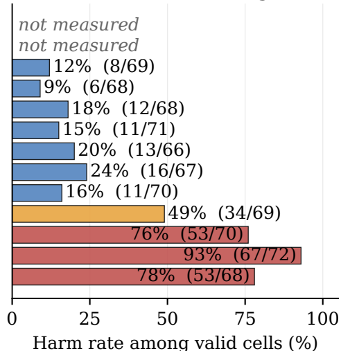
(b) 24-item held-out grid
