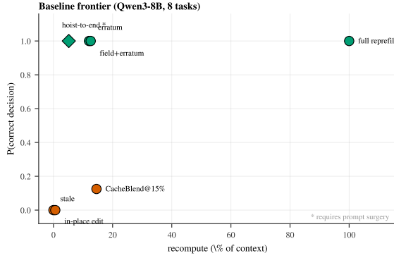
Figure 11: Cost/correctness frontier.
