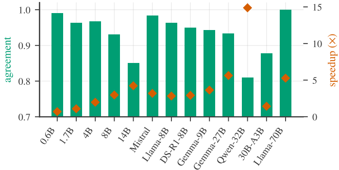
(b) unified edit+compose agent, 13 models (10 domains \times 10 instances; Gemma: 40 traj.)
