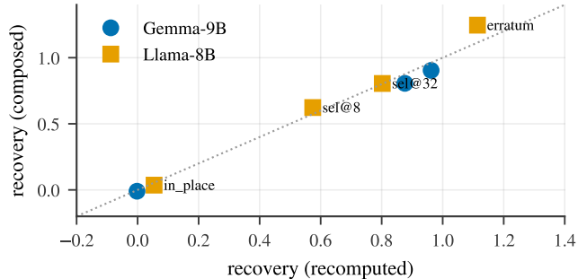
(a) keystone: edit inside a transplant (composed \approx recomputed)
