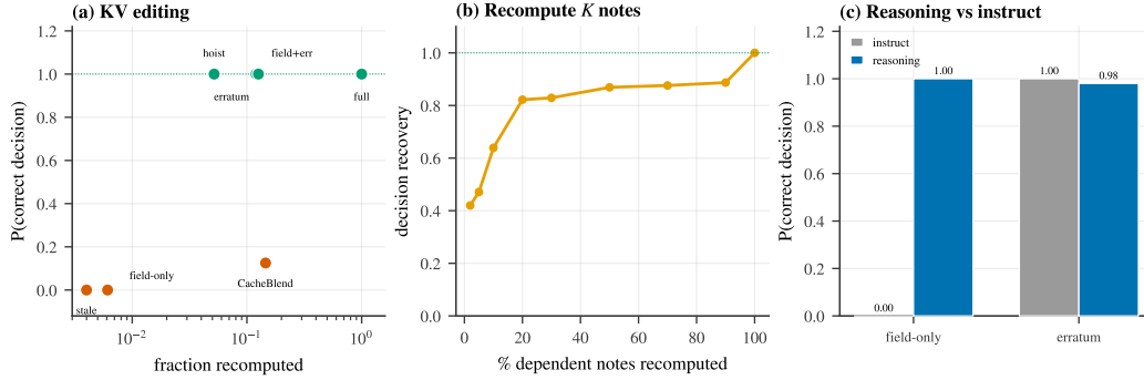
Figure 2: The editable cache, previewed (Qwen3-8B; detail in Sections 3 and 4). (a) KV editing : naive edits (stale, field-only, CacheBlend) fail while erratum, field+erratum, and hoisting reach full-reprefill correctness at a fraction of the recompute. (b) Recompute the K most field-dependent downstream notes : decision recovery climbs as more of the affected notes are recomputed, concentrated in a small suffix. (c) Reasoning vs. instruction-tuned : the near-free field-only edit recovers the decision on a reasoning model (1.00) but is ignored on an instruction-tuned one (0.00); the erratum fixes both.
