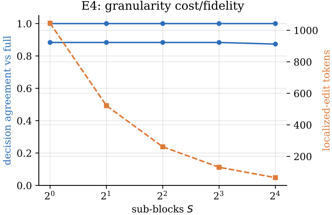
Figure 12: E4 — granularity is a free knob. Splitting memory into S independently-precompiled blocks makes a localized edit S\times cheaper and stays decision-lossless to S=16 ; only genuinely cross-referential facts must be kept in one block (Appendix G).
