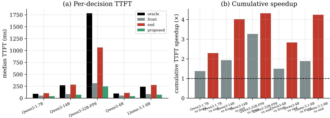
Figure 13: E5 — end-to-end agent. (a) Per-decision median TTFT for the proposed compose+edit agent vs. oracle, front, and end-placement baselines. (b) Cumulative TTFT speedup of 2.3–4.3 \times over repreload-every-turn, growing with model size, at faithful next-token decisions.
