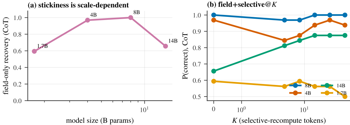
Figure 5: Editing is model-dependent (the editing landscape and the reasoning-vs-instruct split are previewed in Figure 2). (a) The stickiness of the memoized conclusion is model-dependent: the near-free field-only reasoning recovery varies non-monotonically across model sizes. (b) field+selective@K: the minimal recompute K^* to reach full quality is likewise model-dependent.
