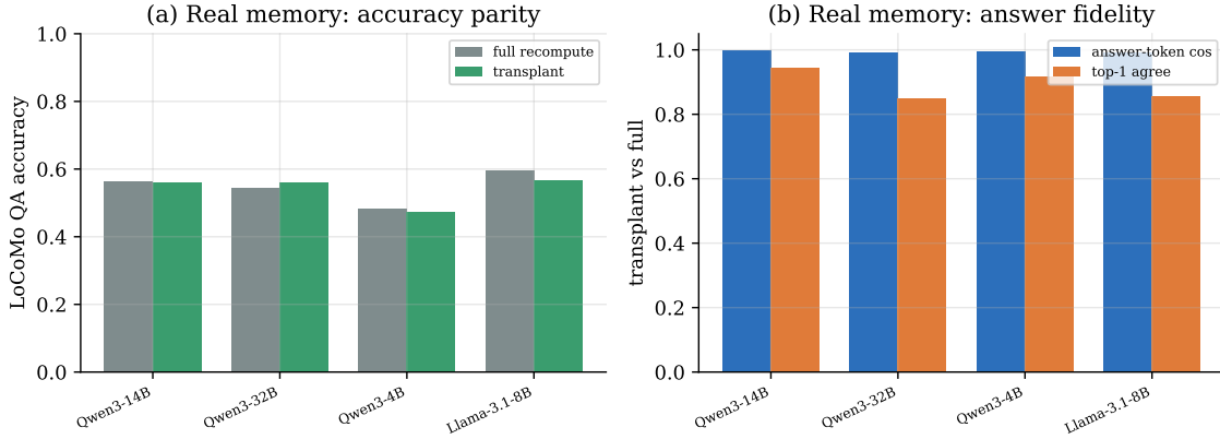
Figure 11: LoCoMo — external validity on real conversations. Over all 1,540 answerable questions per model, transplanting the multi-session dialogue memory is statistically equivalent to full recompute in QA accuracy (TOST) on the Qwen3 models and within 2.7 points on Llama-3.1-8B.
