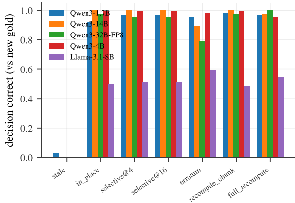
(a) Editing a memory fact (CoT)
