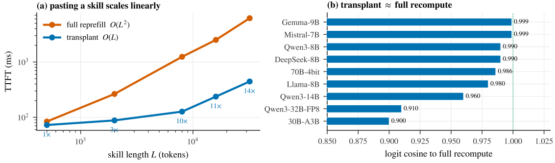
Figure 6: Composing the cache. (a) Pasting a precompiled skill is O(L) vs. full refill’s O(L^2) ; TTFT speedup reaches 13.9\times at 32k tokens. (b) The transplanted skill matches full recompute in next-token logits (cosine 0.90–0.999) across the model family.
