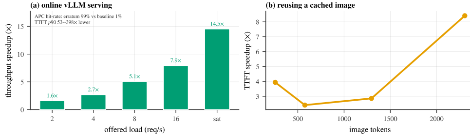
Figure 15: Systems payoff. (a) Online vLLM serving (V1 engine, CUDA graphs, continuous batching, APC, Poisson arrivals): the append-only erratum keeps the prefix cache-aligned (98.5% vs. 1% APC hit-rate), so its throughput advantage grows with offered load—up to 14.5\times at saturation—while p_{90} TTFT is 53–398 \times lower. (b) Reusing a cached image (skipping the vision tower and image-token prefill) accelerates time-to-first-token, more so for larger images.
