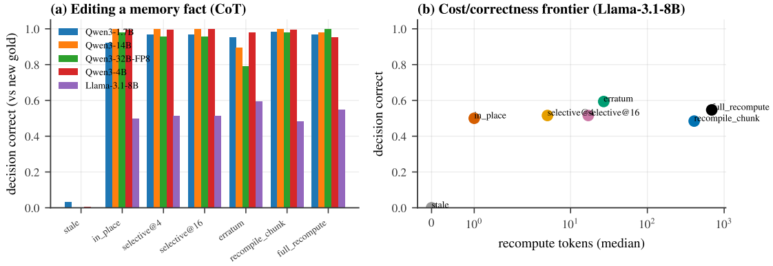
Figure 10: E3 — memory is editable mid-session. Reusing stale memory recovers a toggled fact essentially never; every real edit recovers it. Consistent with Section 4, the near-free in-place edit suffices under chain-of-thought and strengthens with scale , with the append-only erratum as the robust fallback.
