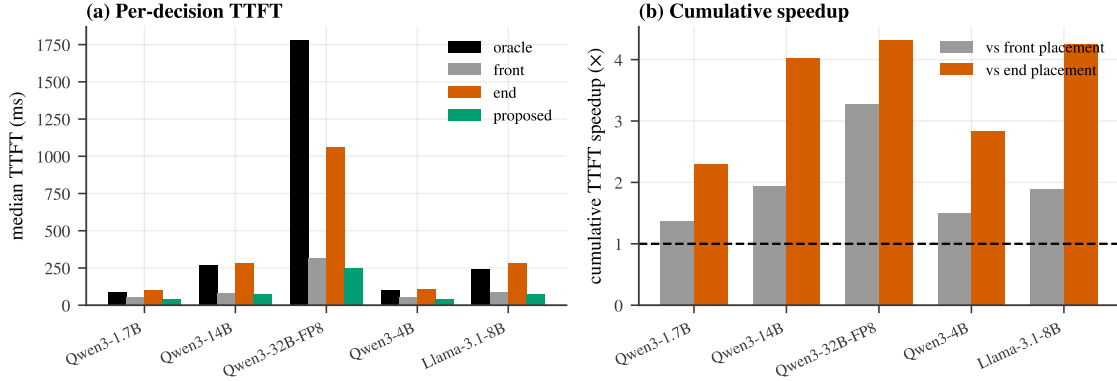
Figure 12: E5 — end-to-end agent. (a) Per-decision median TTFT for the proposed compose+edit agent vs. oracle, front, and end-placement baselines. (b) Cumulative TTFT speedup of 2.3–4.3× over refill-every-turn, growing with model size, at faithful next-token decisions.
