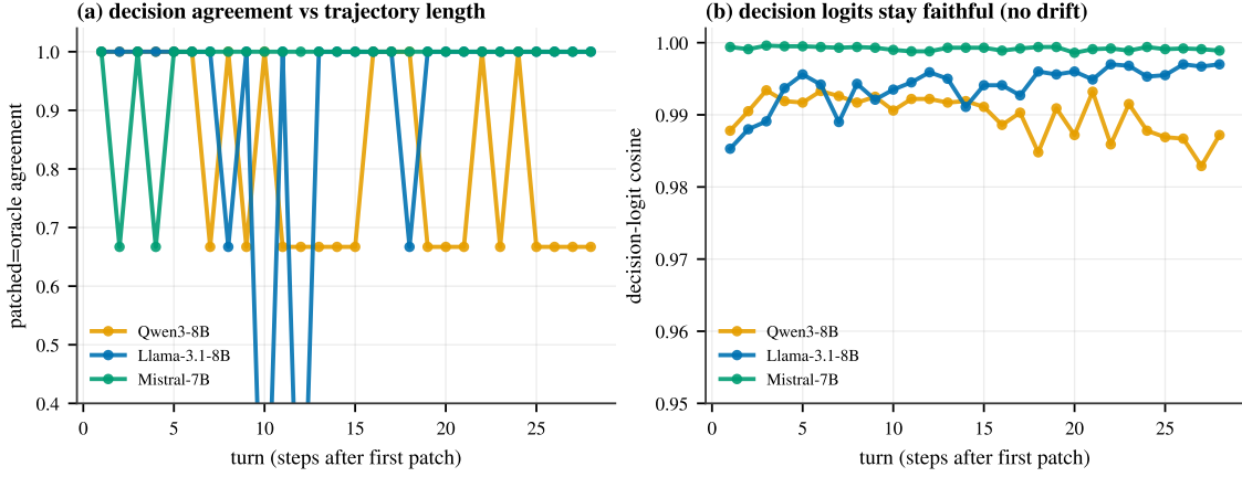
Figure 23: No compounding error over a long trajectory. A gated field toggles every turn for 28 turns; one evolving leave-state+erratum cache vs. full refill of the identical text. (a) Per-turn decision agreement stays high with boundary noise (no downward trend). (b) The decision-logit cosine stays flat at 0.99+—no drift with trajectory length.
