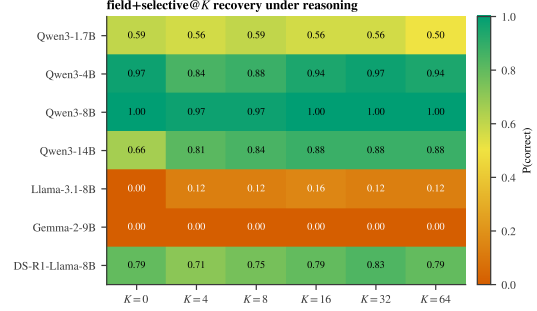
Figure 17: field+selective@K across models.
