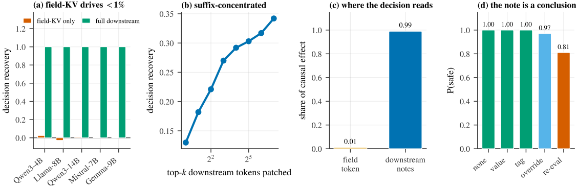
Figure 3: Four causal probes for memoized inference. (a) Refreshing the field’s own KV recovers \approx 0 of the decision; recomputing the downstream recovers it fully. (b) Recovery is suffix-concentrated, accruing only as many post-field tokens are patched. (c) The decision reads almost entirely from downstream notes, not the field token. (d) Once the value is present, override wording is redundant and “re-evaluate” phrasing hurts—the note is a committed conclusion.
