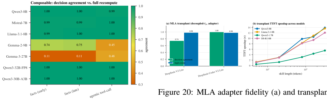
Figure 19: Composable agreement by model \times content type.
