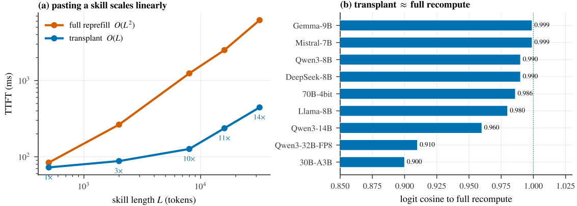
Figure 6: Composing the cache. (a) Pasting a precompiled skill is O(L) vs. full recompile’s O(L^2) ; TTFT speedup reaches 13.9 \times at 32k tokens. (b) The transplanted skill matches full recompute in next-token logits (cosine 0.90–0.999) across the model family.
