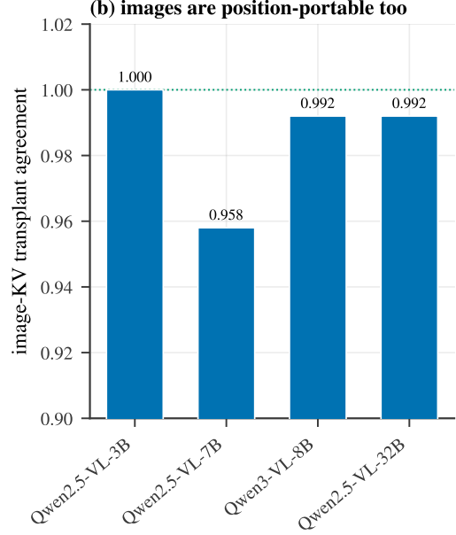
Figure 13: Reach. (a) The substrate is any per-token attention KV cache; we map each attention variant as free / adapter / fixed / partial / open / out-of-scope. (b) Image-KV transplant is near-lossless across vision-language models—images are position-portable too.
