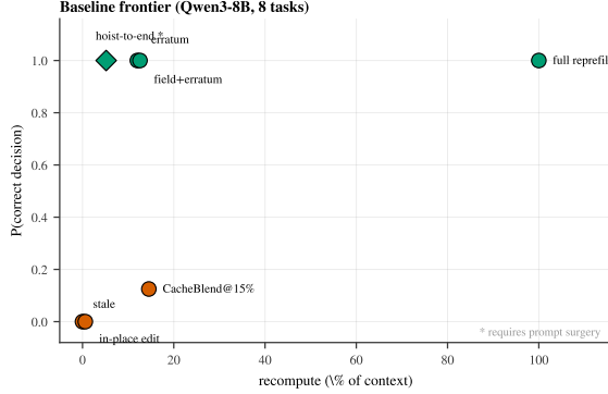
Figure 17: Cost/correctness frontier.
