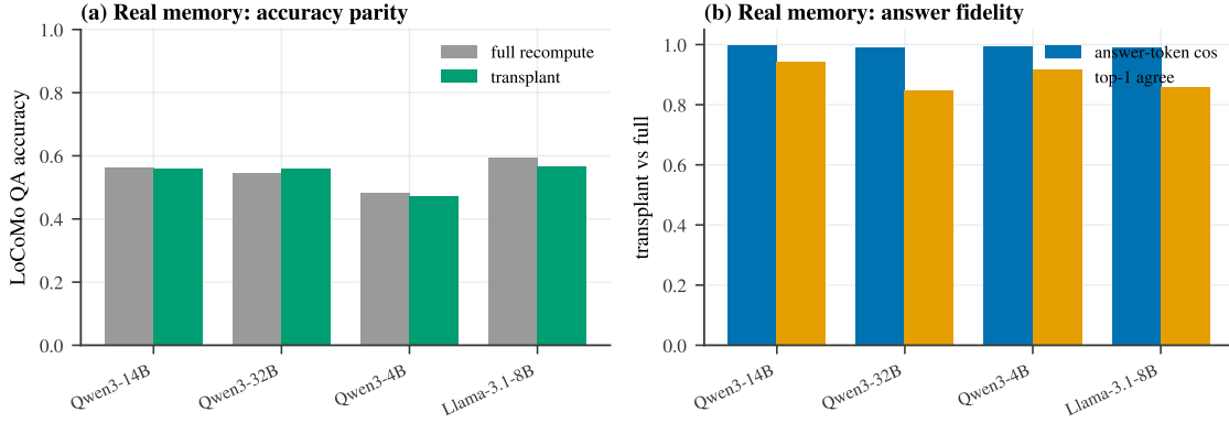
Figure 11: LoCoMo — external validity on real conversations. Over all 1,540 answerable questions per model, transplanting the multi-session dialogue memory is statistically equivalent to full recompute in QA accuracy (TOST) on the Qwen3 models and within 2.7 points on Llama-3.1-8B.
