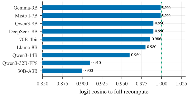
(b) transplant \approx full recompute
