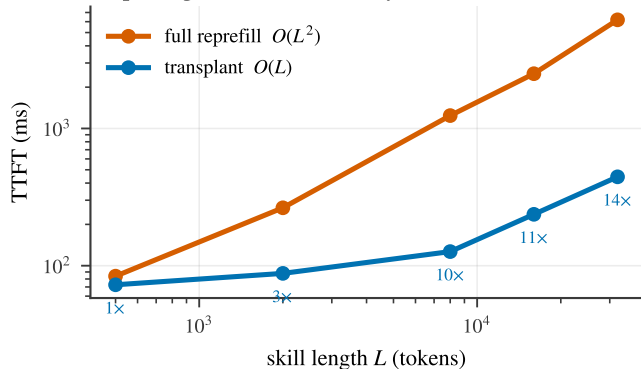
(a) pasting a skill scales linearly
