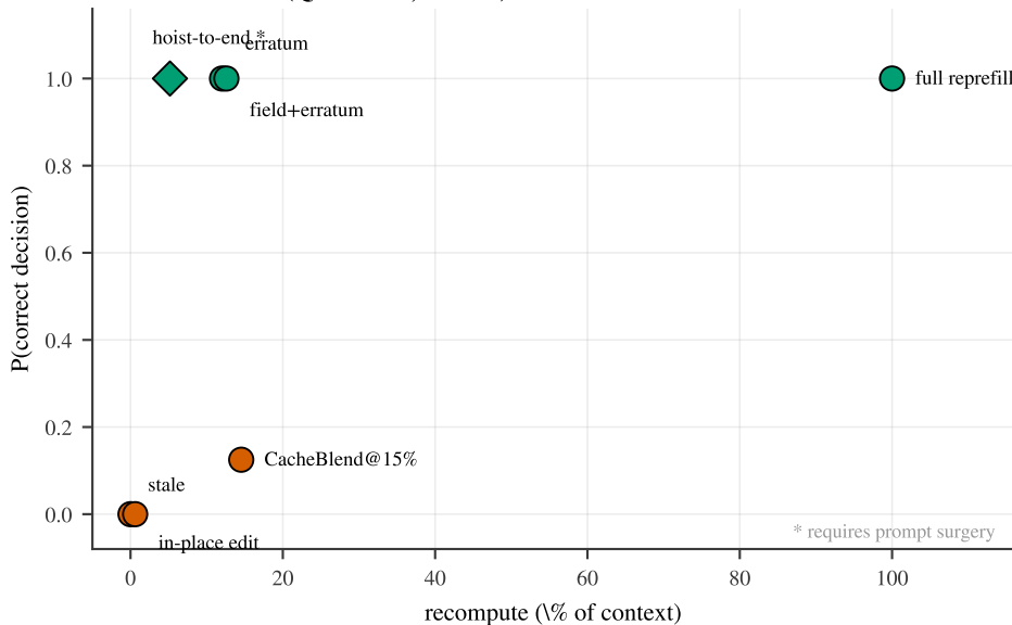
Baseline frontier (Qwen3-8B, 8 tasks)
