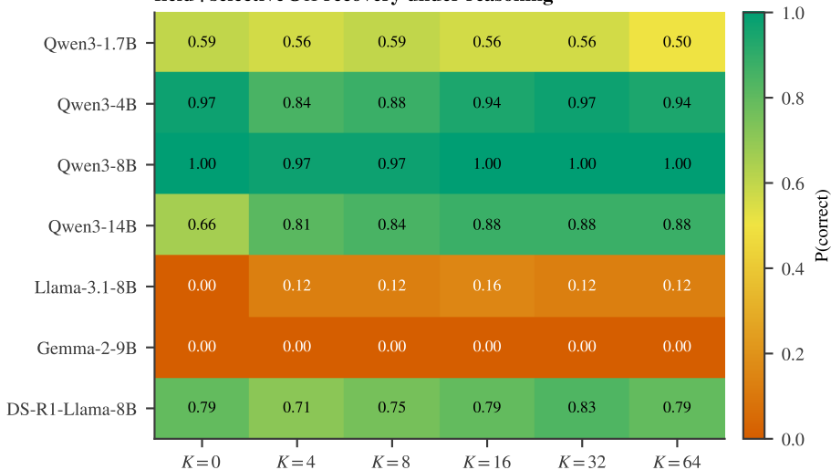
field+selective@K recovery under reasoning
