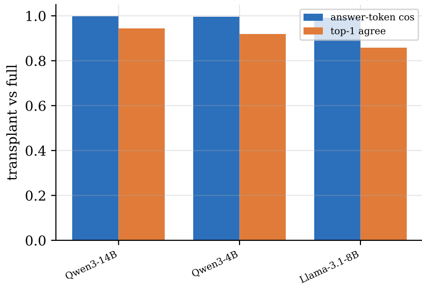
(b) Real memory: answer fidelity
