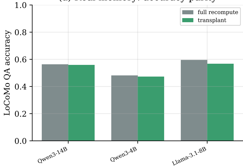
(a) Real memory: accuracy parity
