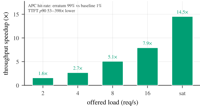
(a) online vLLM serving
