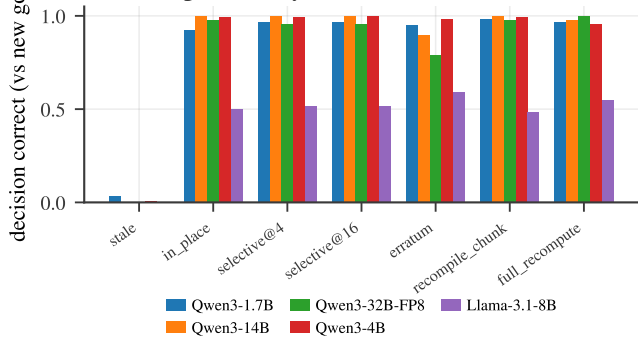
(a) Editing a memory fact (CoT)
