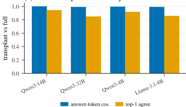
(b) Real memory: answer fidelity
