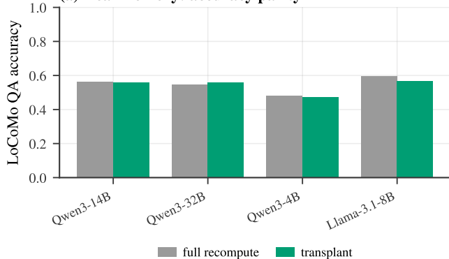
(a) Real memory: accuracy parity
