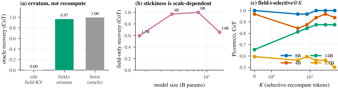
Figure 5: Editing the cache. (a) Editing the field’s KV is ignored; field+erratum reaches the hoist-to-end oracle under CoT. (b) The stickiness of the memoized conclusion is model-dependent, so field-only reasoning recovery varies non-monotonically across model sizes. (c) field+selective@K: the minimal recompute K^* to reach full quality is model-dependent.
