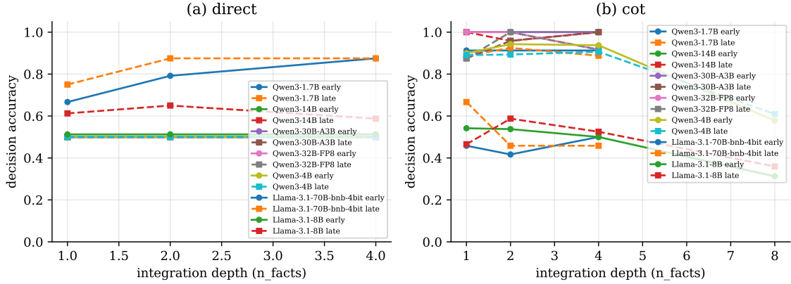
Figure 8: E1 — placement and the pre-digestion cost (Qwen3-4B, CoT). Reading memory late carries a small, statistically significant accuracy cost vs. early that grows with memory length ; late placement is still preferred because it enables O(L) editing/transplant (efficiency quantified in E5).
