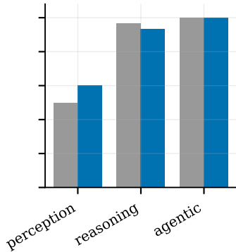
Qwen2.5-VL-7B
