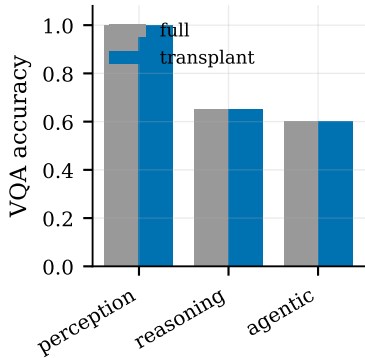
Qwen2.5-VL-3B
