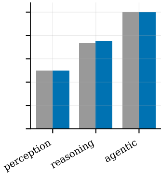
Qwen2.5-VL-32B
