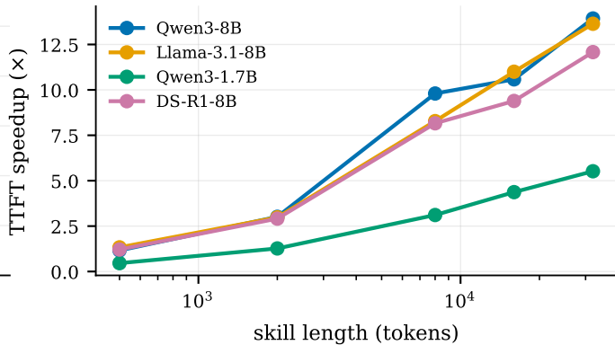
(b) transplant TTFT speedup across models
