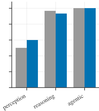
Qwen2.5-VL-7B
