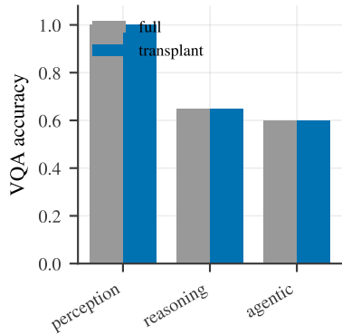
Qwen2.5-VL-3B
