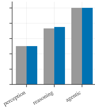
Qwen2.5-VL-32B
